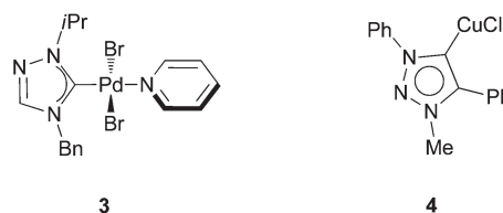
Fig. 1 Catalysts 3 and 4 bearing triazol-based uNHC ligands.
