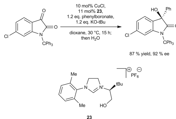
Scheme 11 Copper-mediated arylation of an isatin derivative employing 24 .
