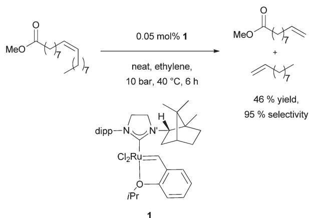
Scheme 1 Ethenolysis of methyl oleate promoted by 1 ( dipp = 2,6-diisopropylphenyl).
