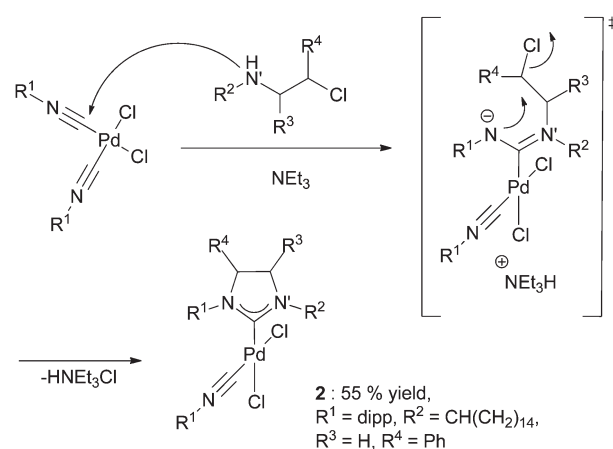
Scheme 2 Variable synthesis of Pd–uNHC complexes in one step.
