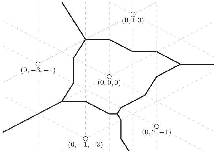
Fig. 8 Tropical Voronoi diagram of five points in \mathbb{R}^3/\mathbb{R}\mathbf{1} . The decomposition of Voronoi regions into semi-polytopes is shown by dashed lines
