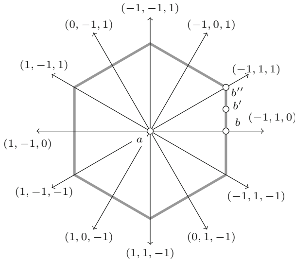
Fig. 7 The bisection fan, \mathcal{F}_{\text{bis}}^d , for d = 2 . The three vectors b - a for Fig. 5 have been marked
