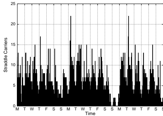
Figure 4: Straddle requirements computed as a moving average of demand assuming both import and export containers reside in the GSI for only 1 hour.
