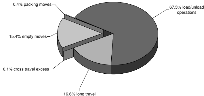
Figure 13: RMG moving time distribution.
