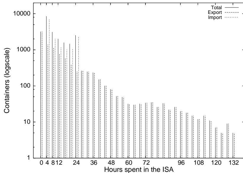
Figure 8: Distribution of ISA dwelling time.
