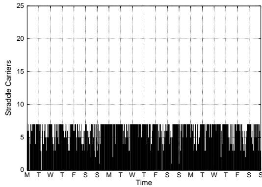
Figure 9: Straddle requirements after Stage 1 optimization with a 24 - 4 = 20 hour effective time window for import containers, and if both import and export containers reside in the GSI for only one hour.
