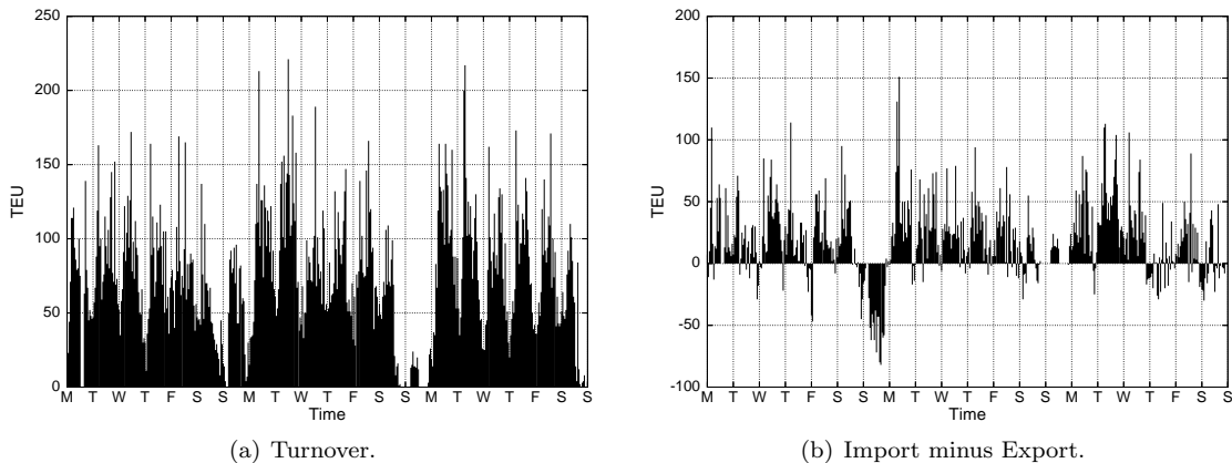
Figure 3: Landside container turnover per hour and dominating transfer direction.
