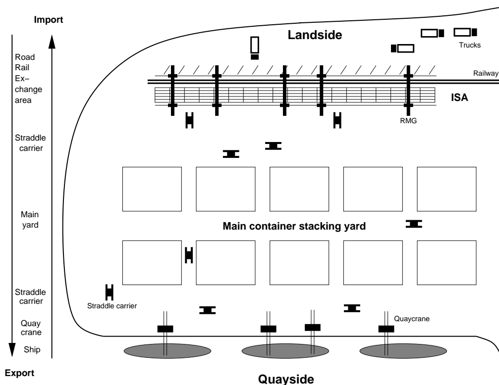
Figure 1: Simplified Port Botany layout
