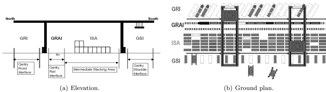
Figure 2: Layout of the container exchange area comprised of the Gantry-Road Interface (GRI), the Gantry-Rail Interface (GRAI), the Intermediate Stacking Area (ISA), and the Gantry-Straddle Interface (GSI).
