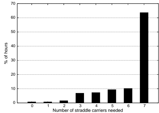
Figure 10: Distribution of straddle fleet utilization.
