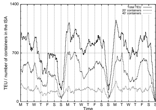
Figure 7: ISA utilization per hour in TEU.
