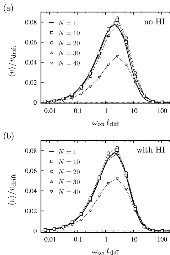
Fig. 3 Rescaled mean velocity \langle v \rangle / v_{\text{drift}} as a function of \omega_{\text{on}} t_{\text{diff}} when particles change their ratchet states simultaneously. Simulation results for different particle numbers N = 1 (solid line), N = 10 ( \square ), N = 20 ( \circ ), N = 30 ( \triangle ), and N = 40 ( \nabla ) are plotted. Parameters are \omega_{\text{off}} t_{\text{drift}} = 3.6 , a = 0.1 , and b = 1 . (a) without hydrodynamic interactions, (b) with hydrodynamic interactions.
