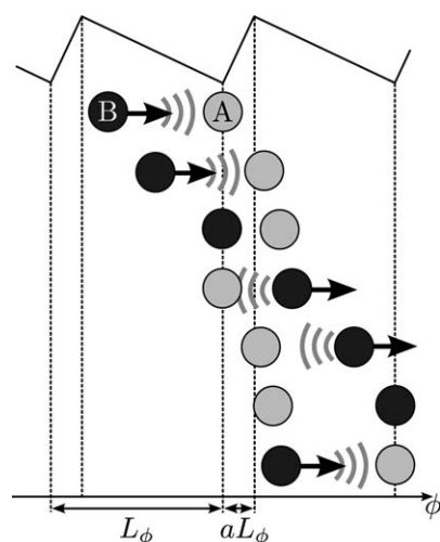
Fig. 8 Transient cluster formation of a pair of particles using hydrodynamic interactions. The front and rear particles are labeled A and B, respectively. The colors of the particles indicate the on-state (black) and the off-state (grey) in the ratchet cycle. The arrows show the drift direction in the ratchet potential and the grey arcs symbolize hydrodynamic interactions between the particles. The picture is explained in detail in the main text.
