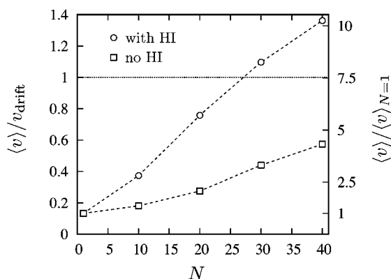
Fig. 6 Mean velocity \langle v \rangle in units of v_{\text{drift}} (left ordinate) and \langle v \rangle_{N=1} (right ordinate) as a function of particle number N . The parameters are \omega_{\text{on}}t_{\text{diff}} = 4.5 , \omega_{\text{off}}t_{\text{drift}} = 3.6 , a = 0.1 , and b = 100 . The symbols refer to simulation results including ( \circ ) and without ( \square ) hydrodynamic interactions, respectively.
