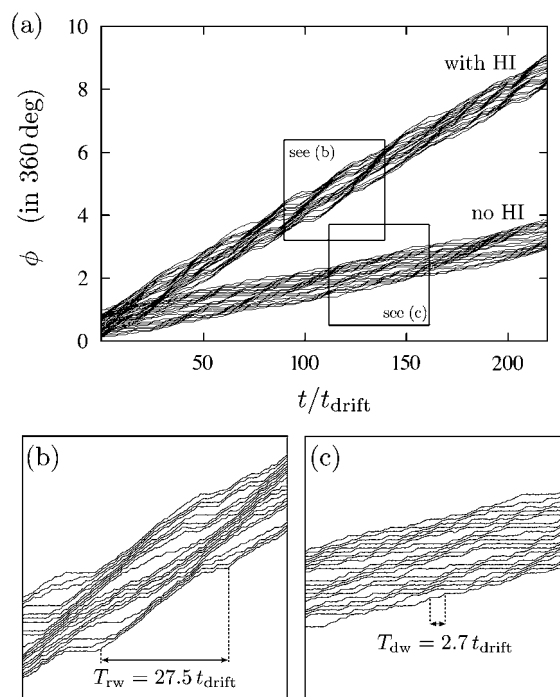
Fig. 7 (a) Particle trajectories \phi(t) of N = 20 particles in the toroidal trap. The upper and lower set of trajectories refer to simulations where hydrodynamic interactions (HI) are included or neglected, respectively. The parameters are a = 0.1 , b = 100 , \omega_{\text{on}}t_{\text{diff}} = 4.5 , and \omega_{\text{off}}t_{\text{drift}} = 3.6 . The boxes indicate close-ups of the trajectories in panels (b) and (c). Examples of the run-walk cycle with duration T_{\text{rw}} and the drift-wait cycle with duration T_{\text{dw}} are indicated in (b) and (c), respectively.
