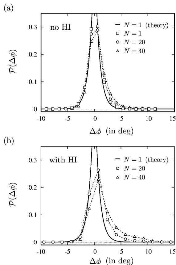
Fig. 5 The probability density function \mathcal{P}(\Delta\phi) for a particle displacement \Delta\phi at the moment when the particle changes to the on-state determined from the same simulation data as the graphs of Fig. 4. The curves belong to particle numbers N = 1 ( \square ), N = 20 ( \circ ), and N = 40 ( \triangle ), and the full line corresponds to the analytic expression of eqn (20) for a single particle. (a) Without hydrodynamic interactions, (b) with hydrodynamic interactions.
