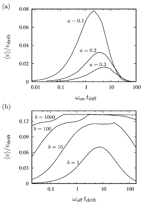
Fig. 2 Rescaled mean velocity \langle v \rangle / v_{\text{drift}} of a single particle, (a) as a function of \omega_{\text{on}} t_{\text{diff}} for a = 0.1, 0.2 and 0.3 with \omega_{\text{off}} t_{\text{drift}} = 3.6 and b = 1 . (b) as a function of \omega_{\text{off}} t_{\text{drift}} for b = 1, 10, 100 and 1000 with \omega_{\text{on}} t_{\text{diff}} = 4.5 and a = 0.1 .
