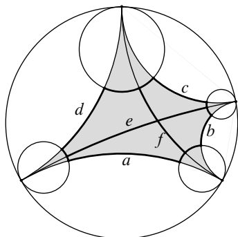
FIGURE 11 Ptolemy relation
