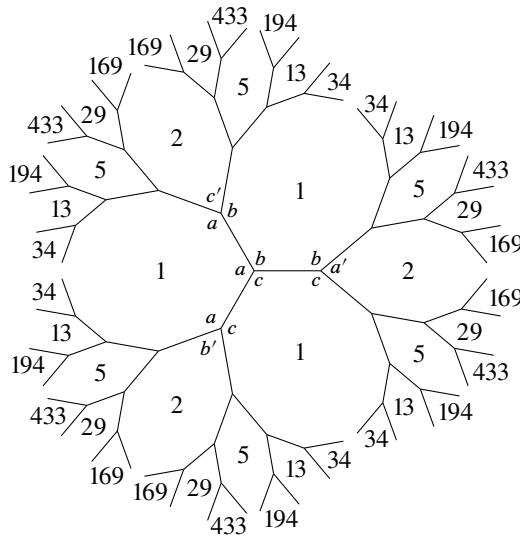
FIGURE 1 Markov tree
