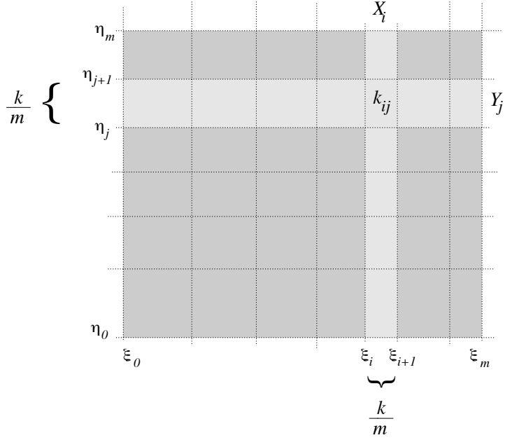
Figure 1: Subdividing the plane into cells
