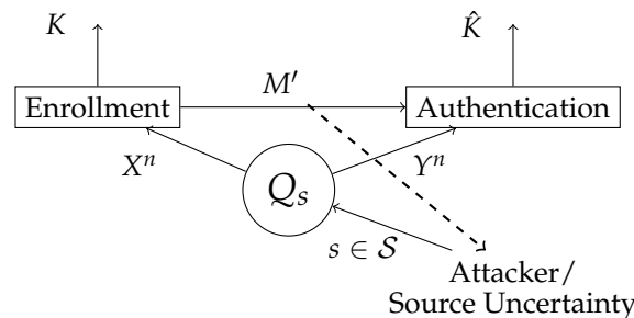
Figure 3. The attacker controls the state of the source s \in \mathcal{S} . The biometric sequences X^n and Y^n are observed at the enrollment and authentication, terminal respectively. In the enrollment terminal, the key K and the helper data M' are generated. The helper data is public, hence the attacker also has access to it. In the authentication terminal, an estimation of a key \hat{K} is made based on the observed authentication sequence Y^n and the helper data M' .
