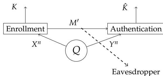
Figure 1. The biometric measurements X^n and Y^n are observed in the enrollment and authentication terminal, respectively. In the enrollment terminal, the key K and the helper data M' are generated. The helper data is public, hence the eavesdropper also has access to it. In the authentication terminal, an estimation of a key \hat{K} is made based on the observed biometric measurements Y^n and the helper data M' .
