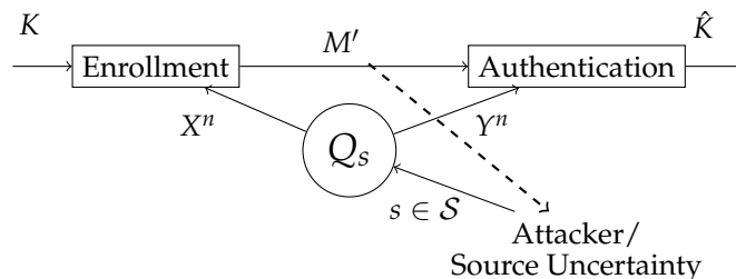
Figure 4. The attacker controls the state of the source s \in \mathcal{S} . The biometric sequences X^n and Y^n are observed in the enrollment and authentication terminal, respectively. In the enrollment terminal, the key K is predefined and the helper data M' is generated. The helper data is public, hence the attacker also has access to it. In the authentication terminal, an estimation of a key \hat{K} is made based on the observed authentication sequences Y^n and the helper data M' .
