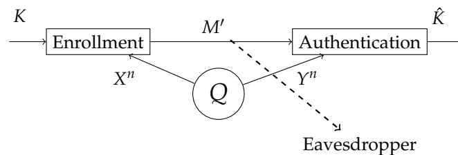
Figure 2. The biometric sequences X^n and Y^n are observed at the enrollment and authentication terminal, respectively. In the enrollment terminal, the helper data M' is generated for a given secret key K . The helper data is public, hence the eavesdropper also has access to it. In the authentication terminal, an estimation of a key \hat{K} is made based on the observed biometric authentication sequence Y^n and the helper data M' .
