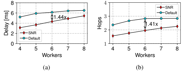
Fig. 4. SNR vs. default. (a) Average delay among the chosen nodes in TopologyZoo networks (b) Average hops among the chosen nodes in TopologyZoo networks
