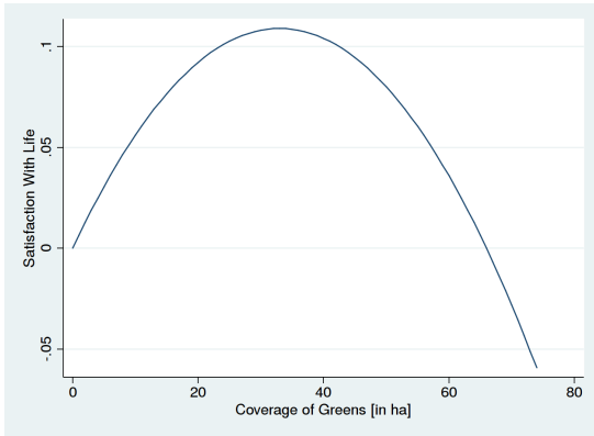
(c) Results - Optimal value of coverage of green urban areas.
