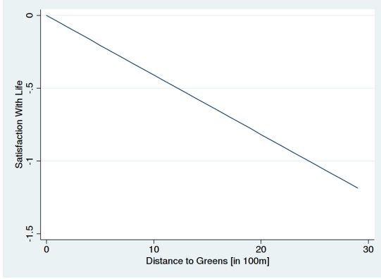
(a) Results - Optimal value of distance to green urban areas.
