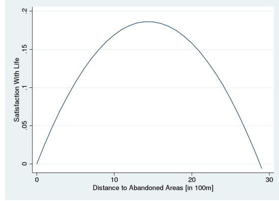
(b) Results - Optimal value of distance to abandoned areas.
