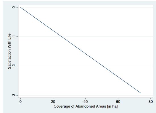
(d) Results - Optimal value of coverage of abandoned areas.
