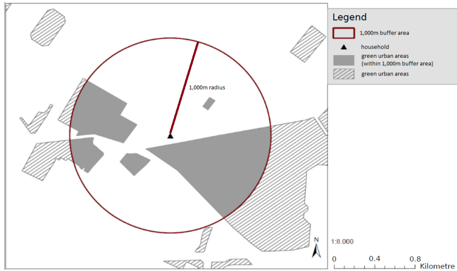
Figure 1: Data - Definition of Coverage
