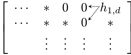
FIG. 6.1. Graphical illustration of the Rotation Lemma. Shown is the upper-right-hand corner of H_d = [H_{d,d-1}, h_d] . We know that H_{d,d-1} is (s + 2) -band Hessenberg with s + 3 < d and that h_{1,d} \neq 0 . We construct an orthogonal transformation G such that the matrix \tilde{H}_d = G^* H_d G remains unreduced upper Hessenberg, while the nonzero entry h_{1,d} \neq 0 is “rotated” to the last column of \tilde{H}_{d,d-1} , so that at least one of its entries \tilde{h}_{1,d-1} and \tilde{h}_{2,d-1} is nonzero.
