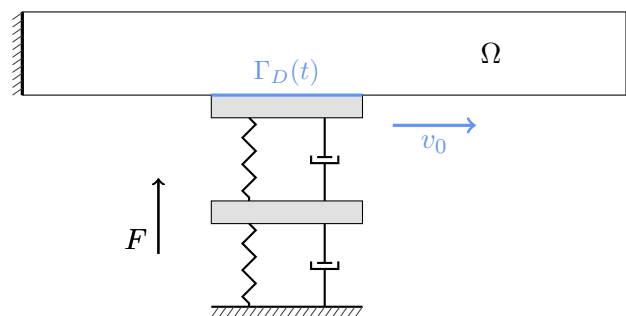
FIGURE 1.1. Example of a flexible body \Omega coupled with a spring damper system along \Gamma_D(t) \subseteq \partial\Omega . The spring damper system moves to the right with speed v_0 . In addition, a force F acts upwards on the spring damper.
