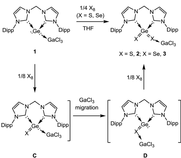
Scheme 2 Synthesis of the bis-NHC and GaCl 3 stabilised monomeric GeS 2 2 and GeSe 2 3 from 1 .
